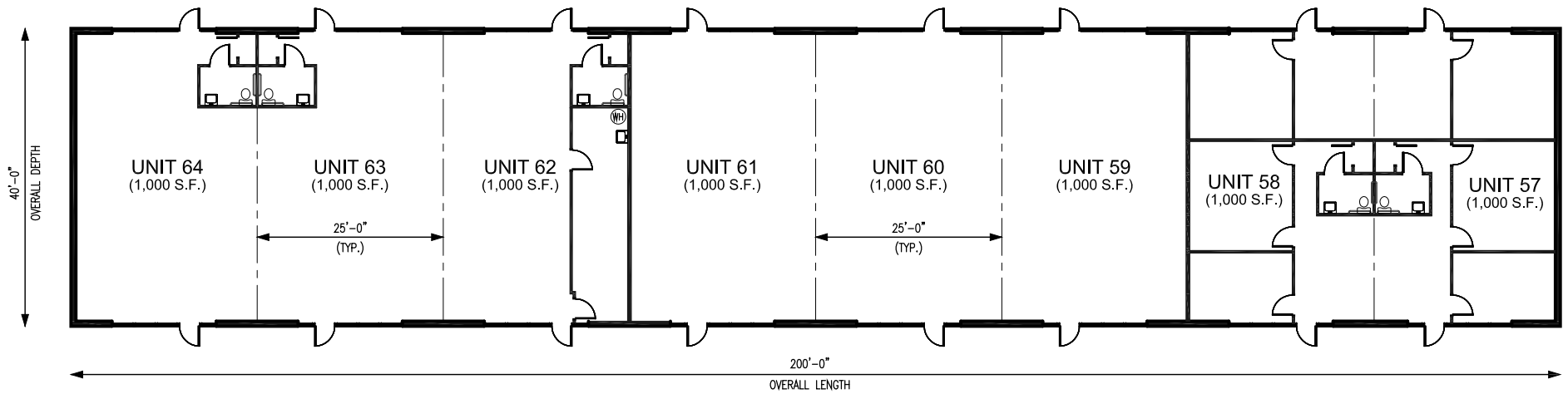
Floor Plan
